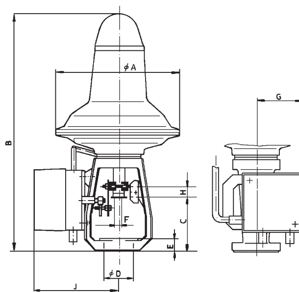
Actuator with indirect function
